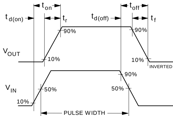
Figure 11. Switching Waveforms.
